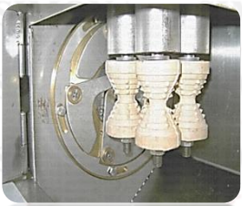
Feeding Rollers (4 pcs.)
